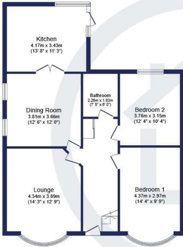
Ground Floor Floor area 91.7 sq.m. (987 sq.ft.)
